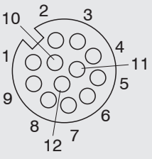
12-pin screw connector, view on solder side (cable)
