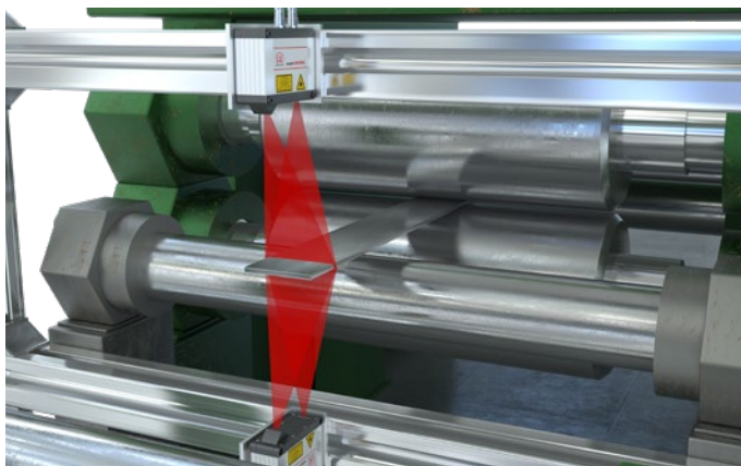
Thickness measurement of cold rolled steel strips
