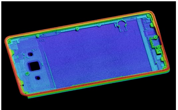
Stitched 3D point cloud of the smartphone carrier plate in 3DInspect
