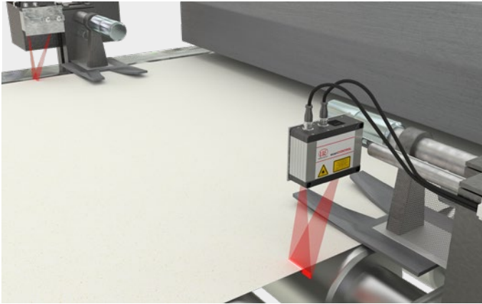
Web monitoring and width measurement with two sensors
